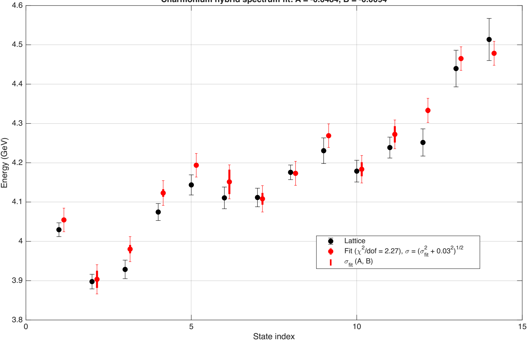
Charmonium hybrid spectrum fit: A = -0.0484, B = -0.0094
